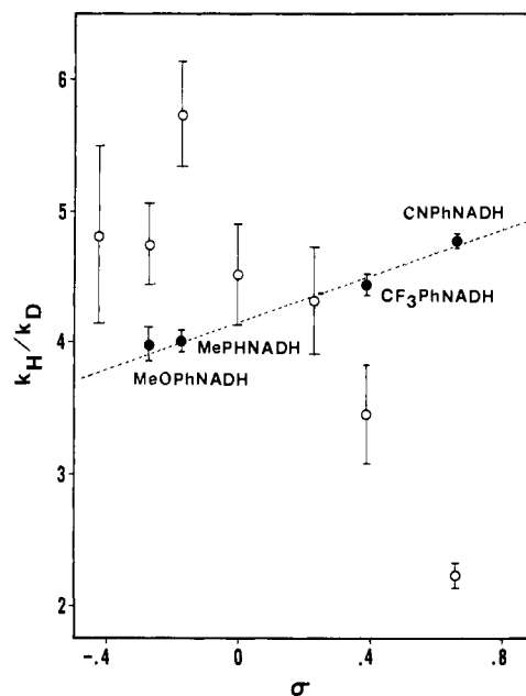
Figure 4. Variation of the kinetic isotope effect determined from the rate ratios of the [\text{H}_2] - and [\text{H},\text{H}] dihydronicotinamides (O) (data from Ohno et al., ref 10) and the [\text{H}_2] - and [\text{H},\text{H}] dihydronicotinamides (●) with the substituent effect ( \sigma ) for reaction of MAI + X-PhNADH in \text{CH}_3\text{CN} at 50 °C. The error bars indicate the standard deviations about each k_{\text{H}}/k_{\text{D}} and were calculated from the square root of the sum of the squares of the errors. The plot shows that the large change in k_{\text{H}}/k_{\text{D}} reported by Ohno et al. 10 is erroneous and that the isotope effects increase with an increase in electronegativity of the substituents.
