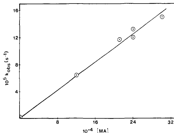
Figure 1. Dependence of k_{\text{obsd}} ( \text{s}^{-1} ) on [\text{MA}] for reaction of labeled N -methylacridinium ion with an excess of N -methylacridin in \text{CH}_3\text{CN} at 30^\circ\text{C} . The least-squares line has a slope of 0.051 \pm 0.002 \text{ M}^{-1} \text{ s}^{-1} .
